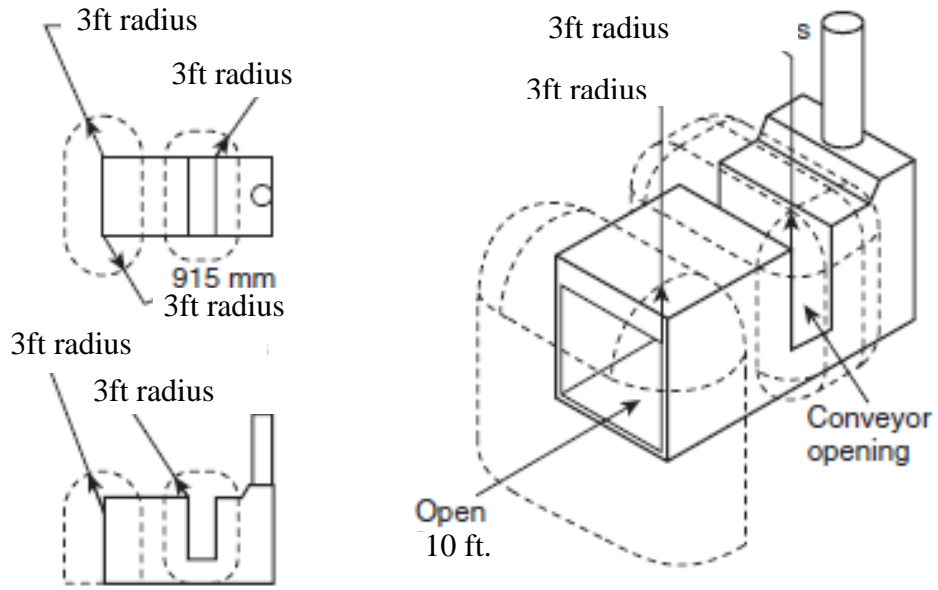
FIGURE 6.5.2 Class I, Division 2; Class I, Zone 2; Class II, Division 2; or Zone 22 Locations Adjacent to an Open-Face or Open-Front Spray Booth or Spray Room
